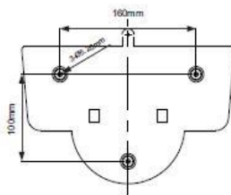
Ceiling Plate
