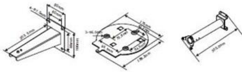
Wall Bracket
