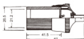
K320890 Auto plug to micro USB/B plug W/fuse W/retractable extension cable (L=500mm) W/short circuit protection In:12V/24V Out:5V 2.1A
