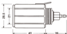
K32088 Auto plug to 2 x USB/A adapter W/fuse W/short circuit / over voltage / reverse protection W/LED In:12V/24V Out:5V 2.1A
