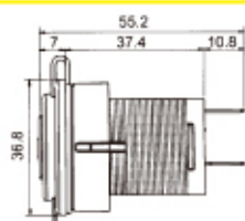
K3210 Auto plug to auto double jack W/light ring W/fuse/10A
