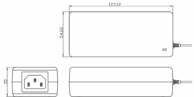
Mechanical Drawing:
