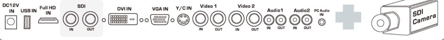
SDI Camera
