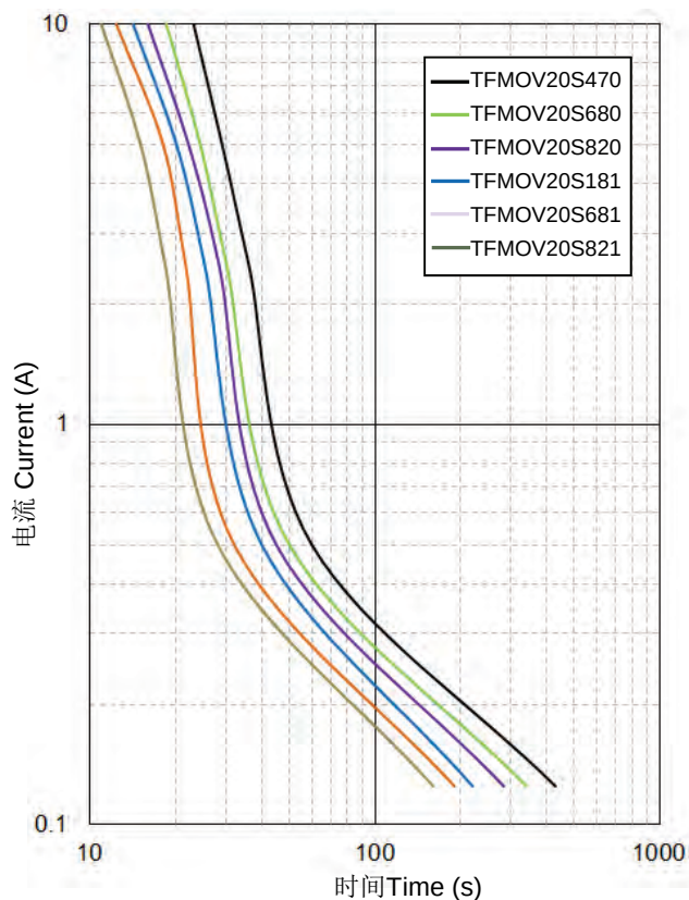
受限电流测试曲线 (UL 1449第3版 39.4条款) Limited Current Test Curve (UL 1449 3rd clause 39.4)
