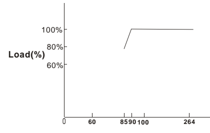
Input Voltage(VAC) Typical static characteristics
