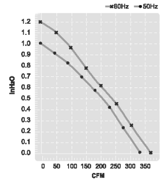
(Roof Fan)
