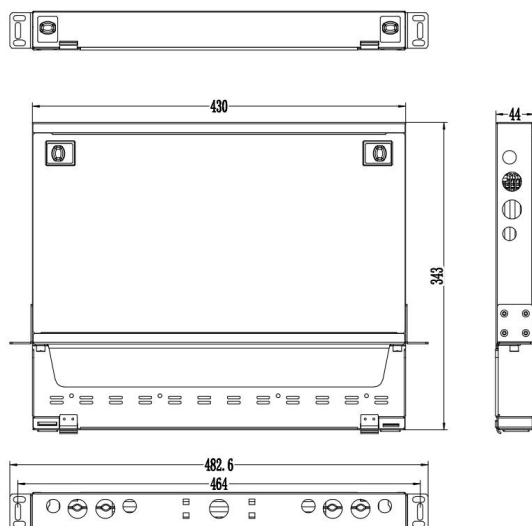
Racks: TK-HRF-1096F
