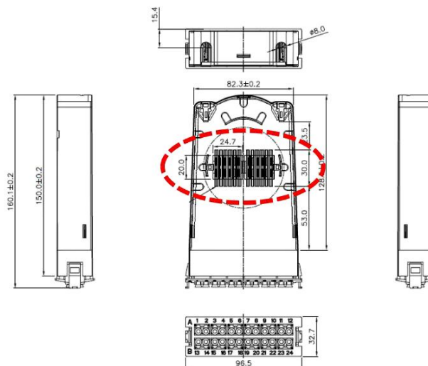
Cassette module: TK-HRM-04
