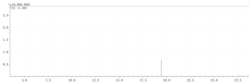
GCMS TIC
