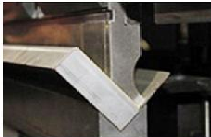
BENDING
