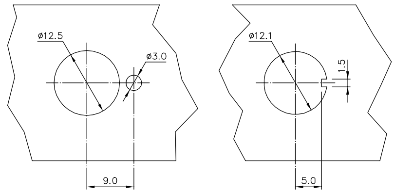
PANEL LAYOUT
