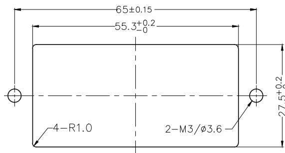
PANEL CUT-OUT
