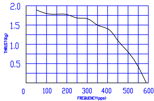
□ PULSE-THRUST CHARACTERISTICS
