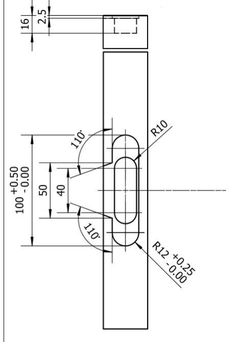
Hole Dimension on the Door Frame
