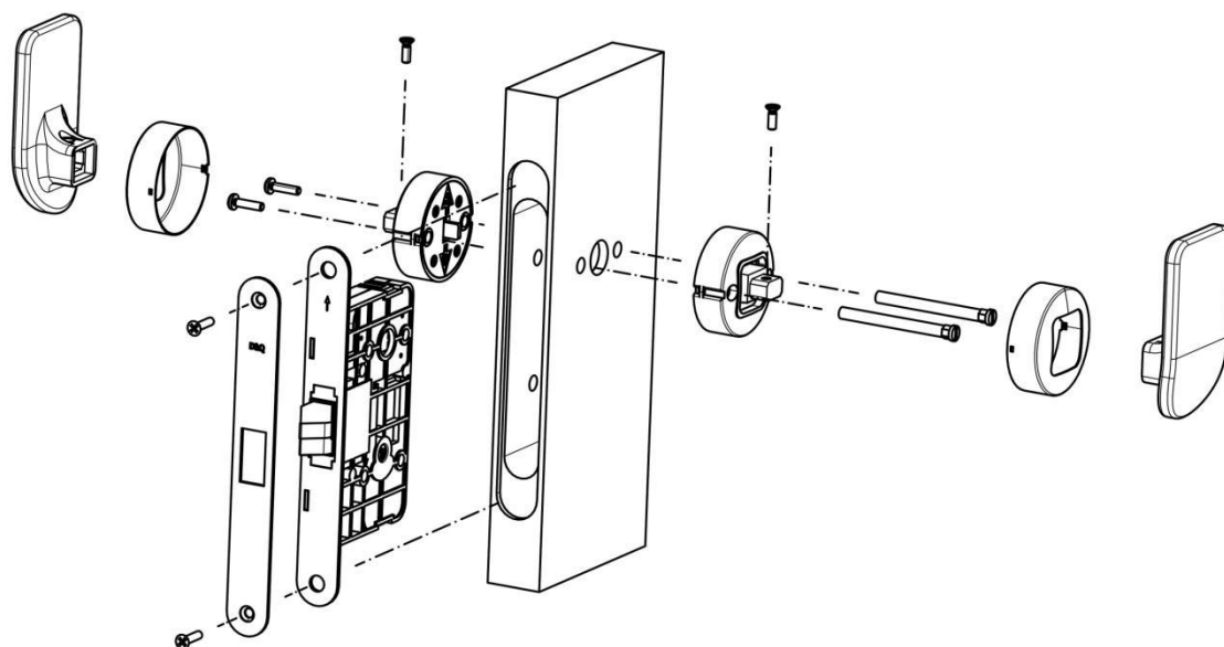
Fitting Instruction
