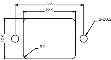
PANEL CUT-OUT
