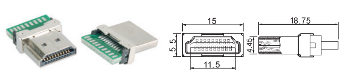
Y99065 19P HDMI socket (SMD)
