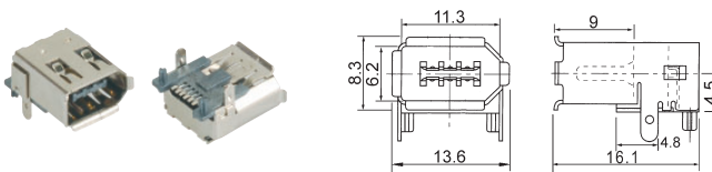
Y99053 6P IEEE 1394 socket right angle
