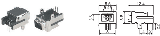
Y99048 4P IEEE 1394 plug (assembly type)
