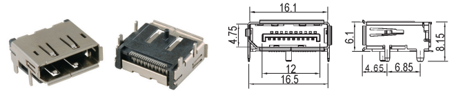
Y990549 DisplayPort socket right angle
