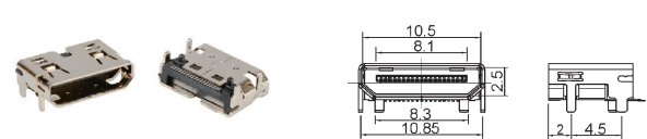
Y99061 19P HDMI plug
