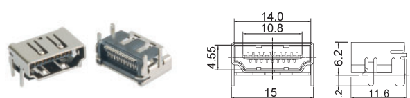
Y99071 19P HDMI socket right angle
