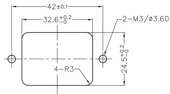
PANEL CUT-OUT
