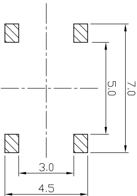
P.C.B LAYOUT TOP VIEW
