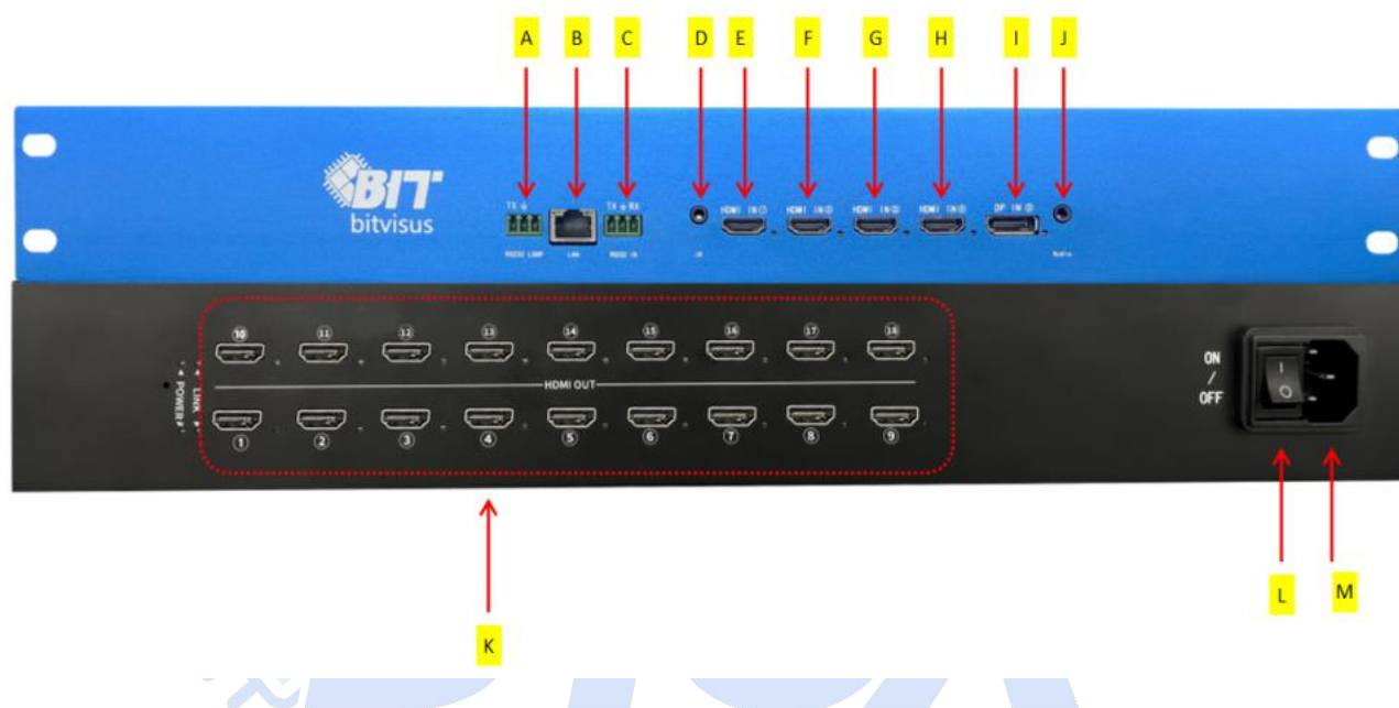
BIT_V418R front panel
