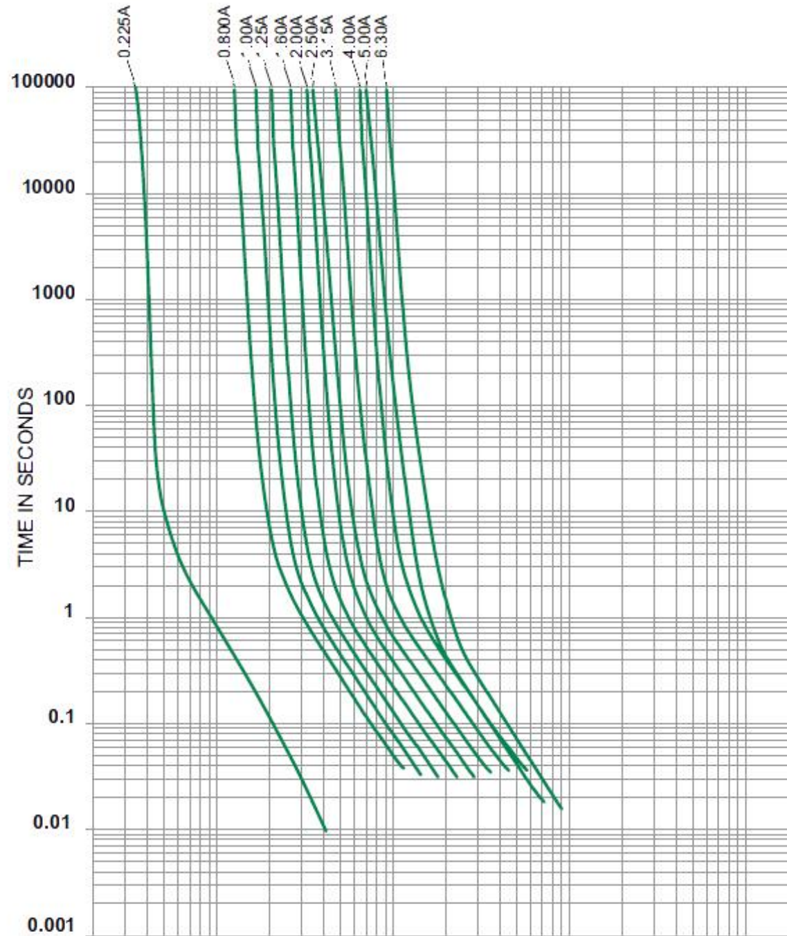
Slow Blow, Average Time vs. Current Curves
