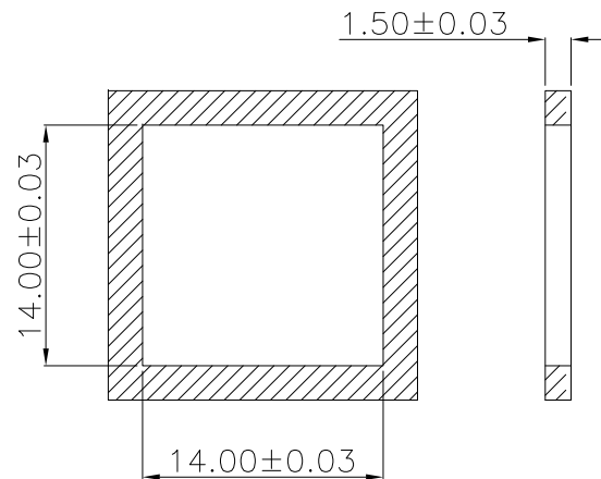
Mounting Plate
