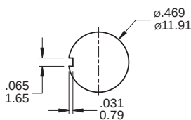
Without locking ring (Keyway)
