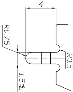
DETAIL A
