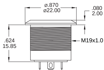
Double flat
