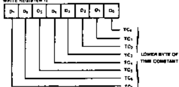
WRITE REGISTER 12
