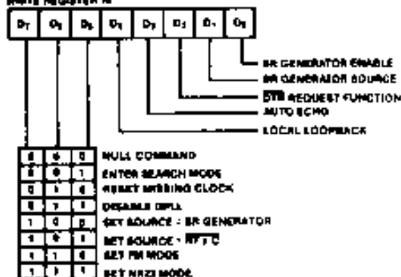
WRITE REGISTER 14
