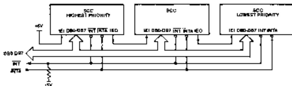
Figure 8. Daisy Chaining SCC's
