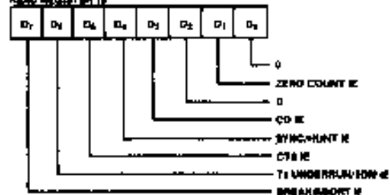
READ REGISTER 15
