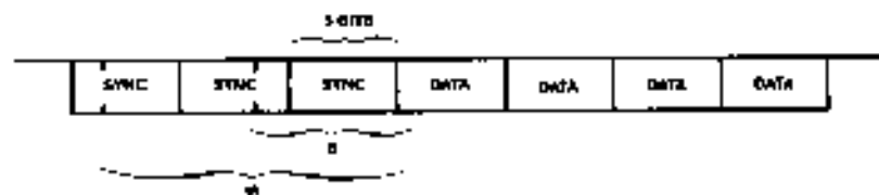
Figure 5. Detecting 5- or 7-Bit Synchronous Characters
