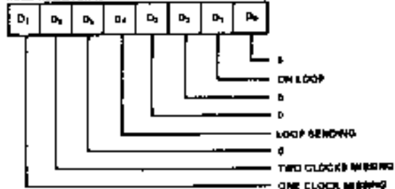
READ REGISTER 10
