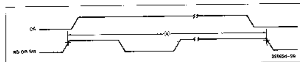
Figure 17. Cycle Timing
