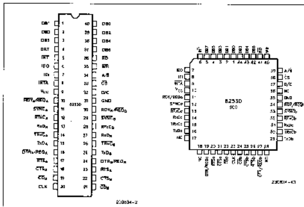
Figure 2. Pin Configurations
