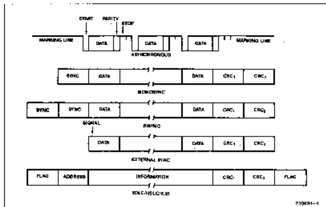
Figure 4. SCC Protocols
