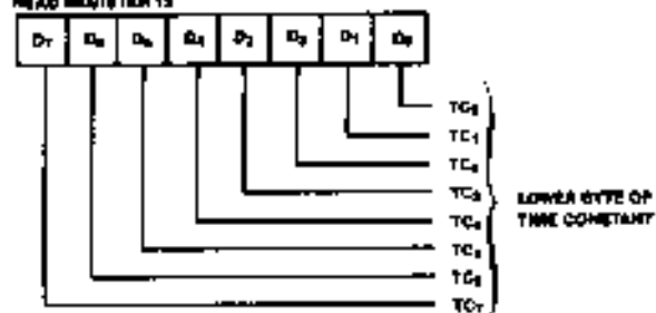
READ REGISTER 13
