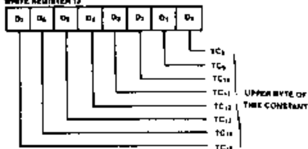
WRITE REGISTER 13
