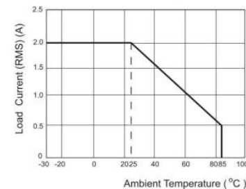
Max. Load Current vs. Ambient Temperature
