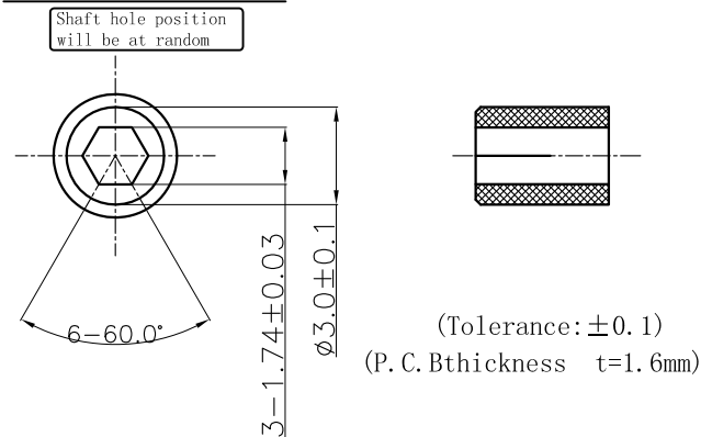
Detail E(2:1) Shaft hole shape and dimension
