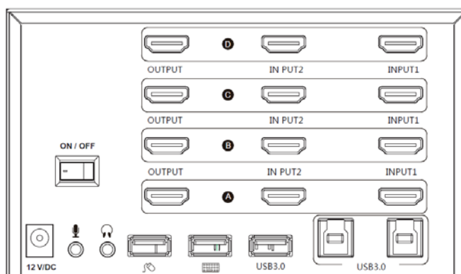
Figure 2 shows the rear panel of HM-KVM2-4
