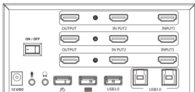
Figure 2 shows the rear panel of HM-KVM2-3
