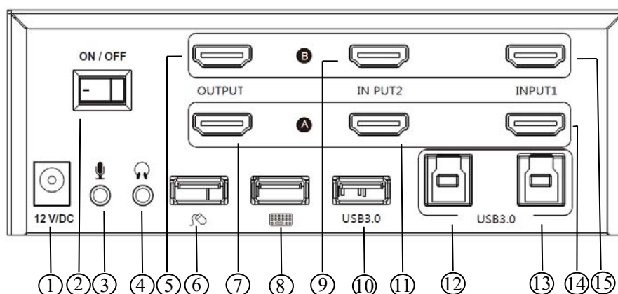
Figure 2 shows the rear panel of HM-KVM2-2
