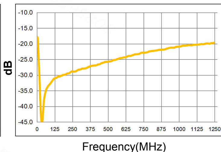
Output Return Loss (Pin4)
