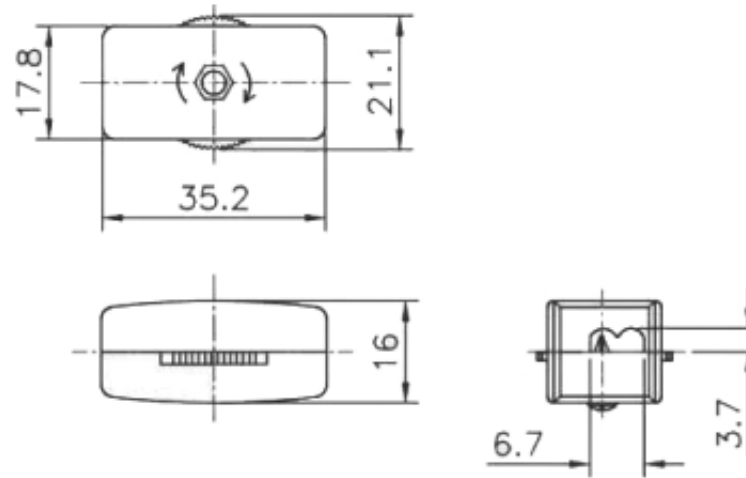
KS-30-2 fitting SPT-2
