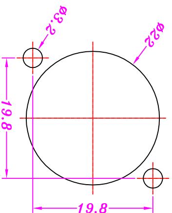
Panel cut out (rear side)
