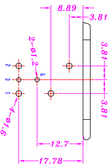
PCB-Layout (component side)
