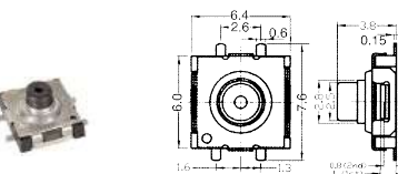
B17223 Tact switch 12V 0.05A
