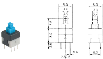
B1719 Tact switch 12V 0.05A
