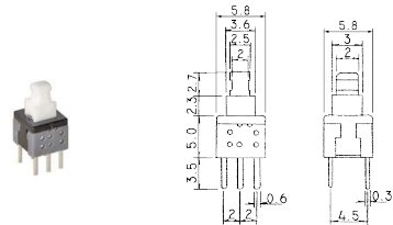
B17173 6 x 6mm Square cover for B17223
