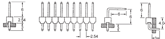
Pin header single row (right angle) YVRxx
