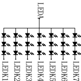
1. LED Diagram:
