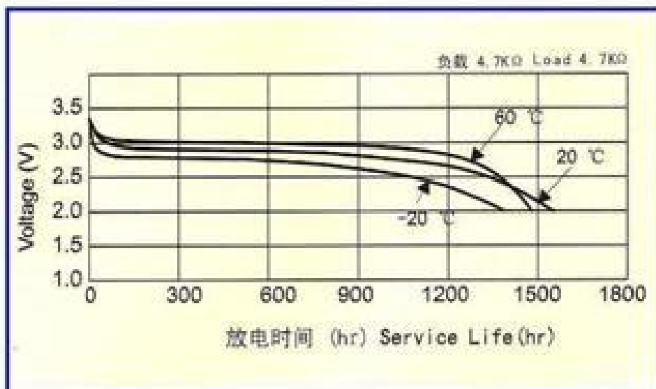
Temperature Characteristics
