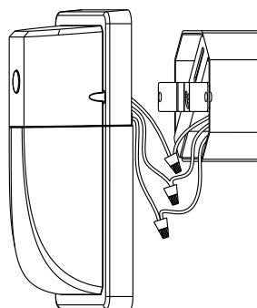
✕ 3. Connect wire
