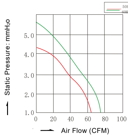
Air Flow vs Air Pressure
