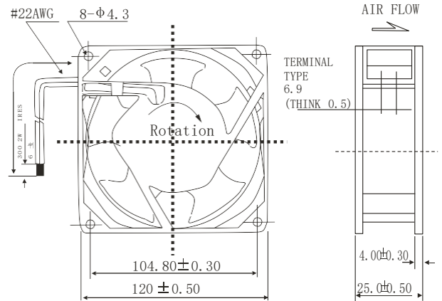
Dimensions (mm)
