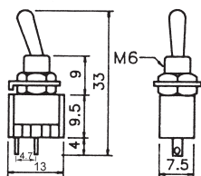
B068A 2P mini toggle switch W/cap (SPST) on-off gold-pin 120V 5A (250V 2A)
