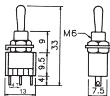
B068C 3P mini toggle switch W/cap (SPDT) on-off-on gold-pin 120V 5A (250V 2A)
