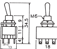
B068H 9P mini toggle switch W/cap (3PDT) on-on gold-pin 120V 5A (250V 2A)
