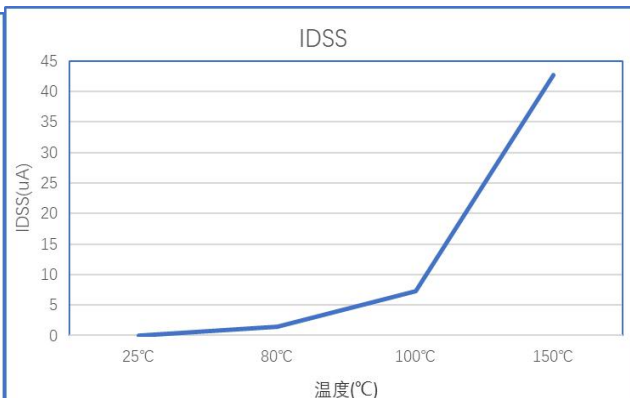
Figure 4 I DSS VS Temperature
