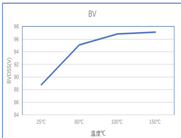
Figure 1 BV DSS VS Temperature
