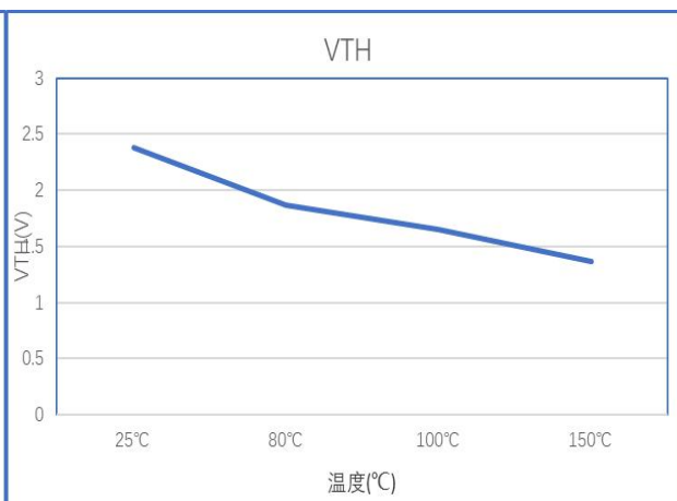
Figure 2 V TH VS Temperature
