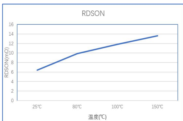
Figure 3 R dson VS Temperature
