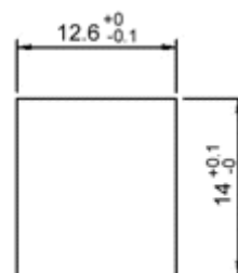
PANEL CUT-OUT THICKNESS: 1.0~1.2mm
