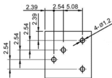
PCB MOUNTING HOLE
