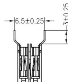
Type 01 A=6.50
