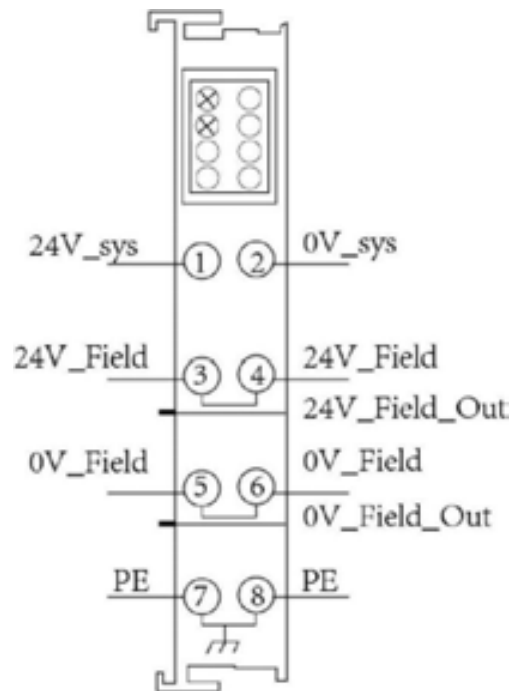
Figure 2.8 GCAN-PLC-400, Power terminal block
