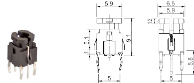
B173840 Illuminated tact switch 12V 0.05A
