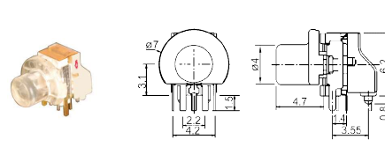
B173850 Illuminated tact switch 12V 0.05A
