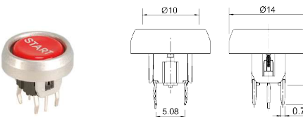
B173820 Illuminated tact switch 12V 0.05A W/white LED
