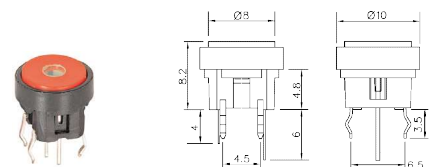
B1737 Illuminated tact switch 12V 0.05A
