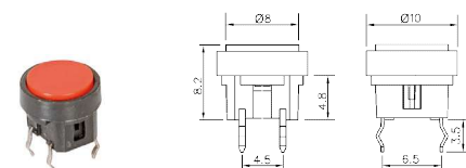
B1735 Tact switch W/O LED 12V 0.05A
