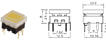
B173821 Illuminated tact switch 12V 0.05A
