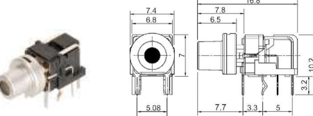
B173855 Illuminated tact switch 12V 0.05A
