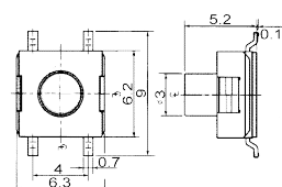
B173342 Sealed tact switch 24V 0.05A Can reach to IP67
