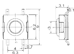
B173340 Sealed tact switch 24V 0.05A Can reach to IP67
