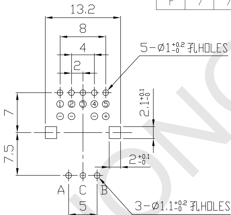
P.C.B.MOUNTING DETAIL
