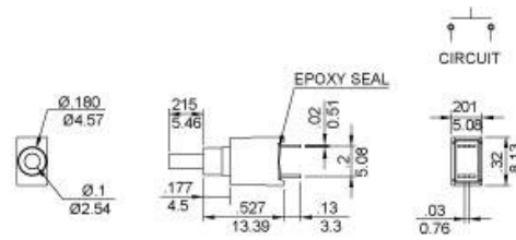
ES-21-C (WITHOUT BRACKET)
