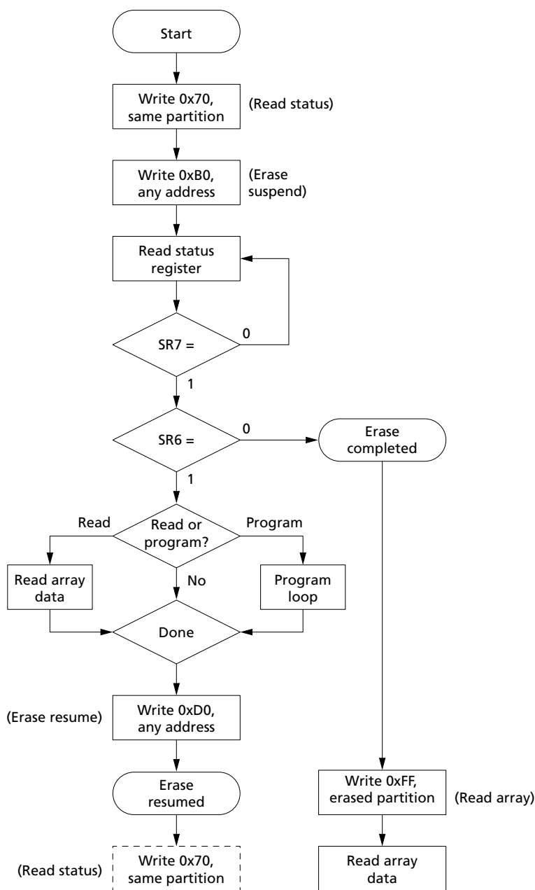
Figure 33: Erase Suspend/Resume Flow Chart
