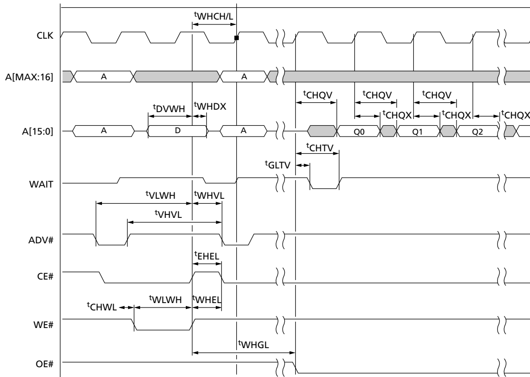
Figure 25: Write to Sync Read (A/D-MUX)
