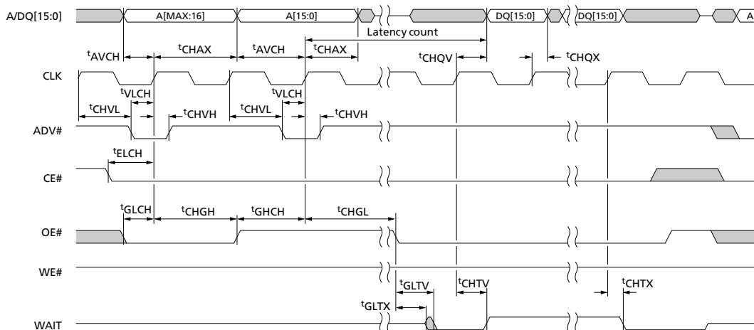
Figure 43: AADM Synchronous Burst READ Cycle (ADV# De-asserted Between Address Cycles)
