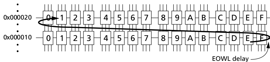
Figure 6: End-of-Wordline Delay
