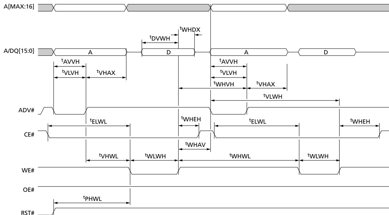
Figure 20: Write Timing
