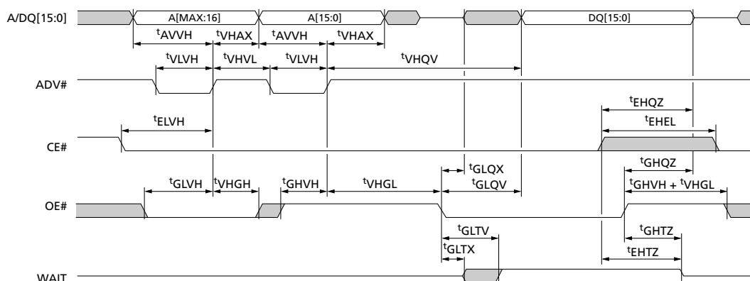
Figure 39: AADM Asynchronous READ Cycle (Latching A[ MAX:0 ])
