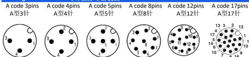
Pin assignment front view/针位分布前视图
