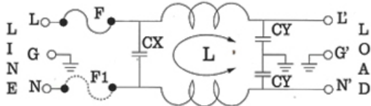
F1:optional fuse ELECTRICAL SCHEMATIC 11
