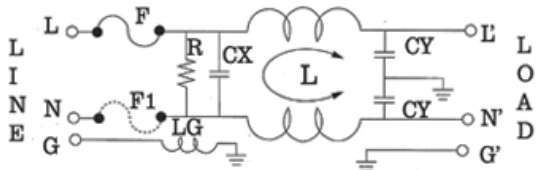
F1:optional fuse ELECTRICAL SCHEMATIC 6
