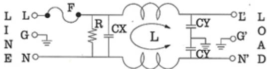
ELECTRICAL SCHEMATIC 5
