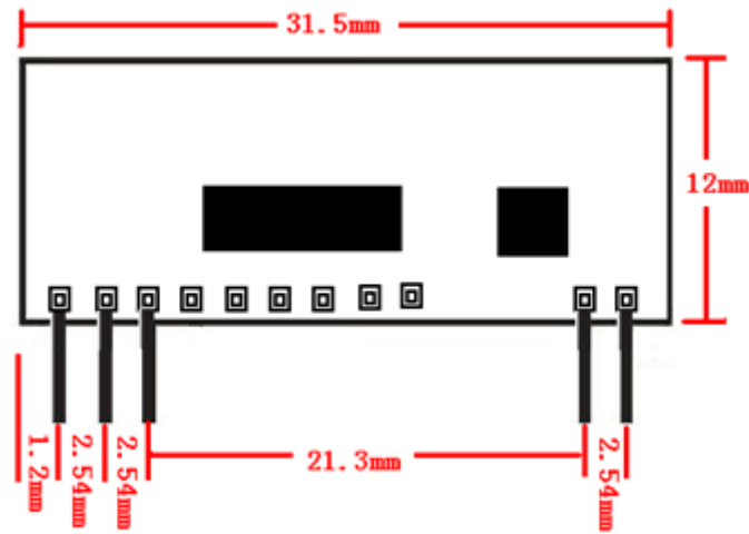
Figure2 CY121 Dimension
